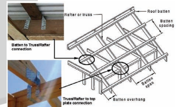
Typical roof connections – Part of image from AS1684
